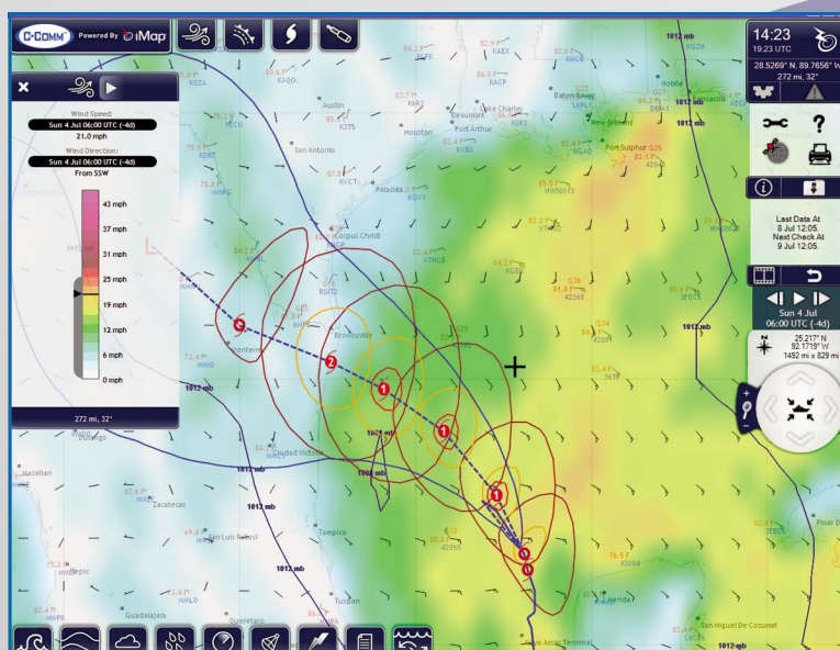
The C-Comm Weather display allows the user to select specific data to be shown, such as hurricane tracking, wind speed/direction and barometric pressure.
